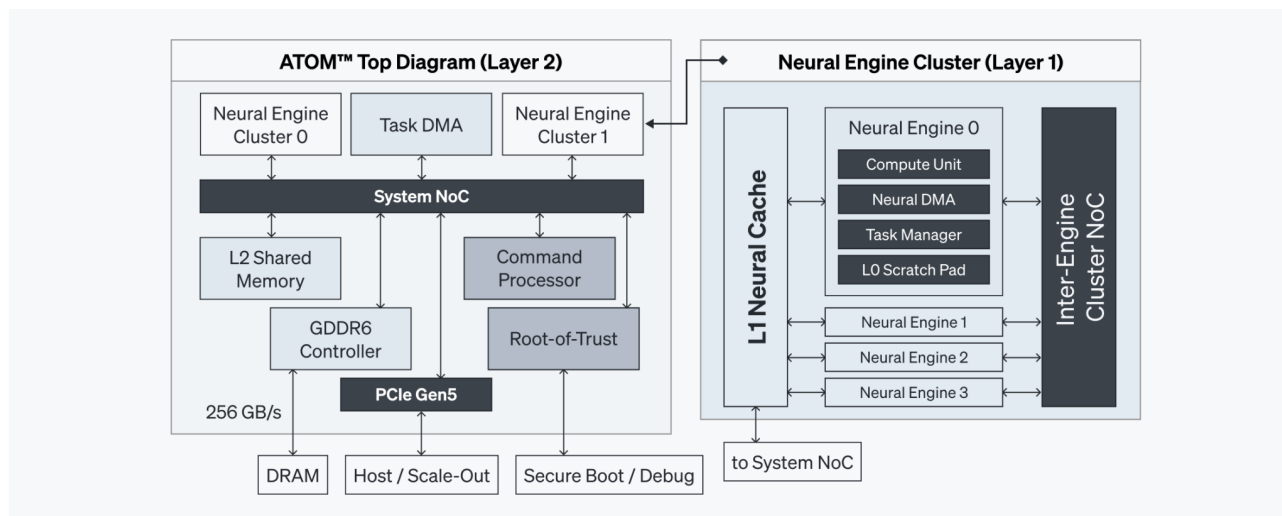
[Figure 1. ATOM™ Multi-layered SoC Architecture]
