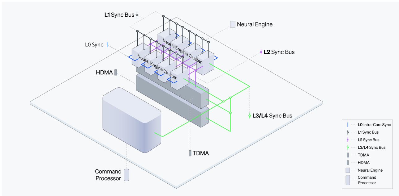
[Figure 4. ATOM™ Synchronization Scheme]
