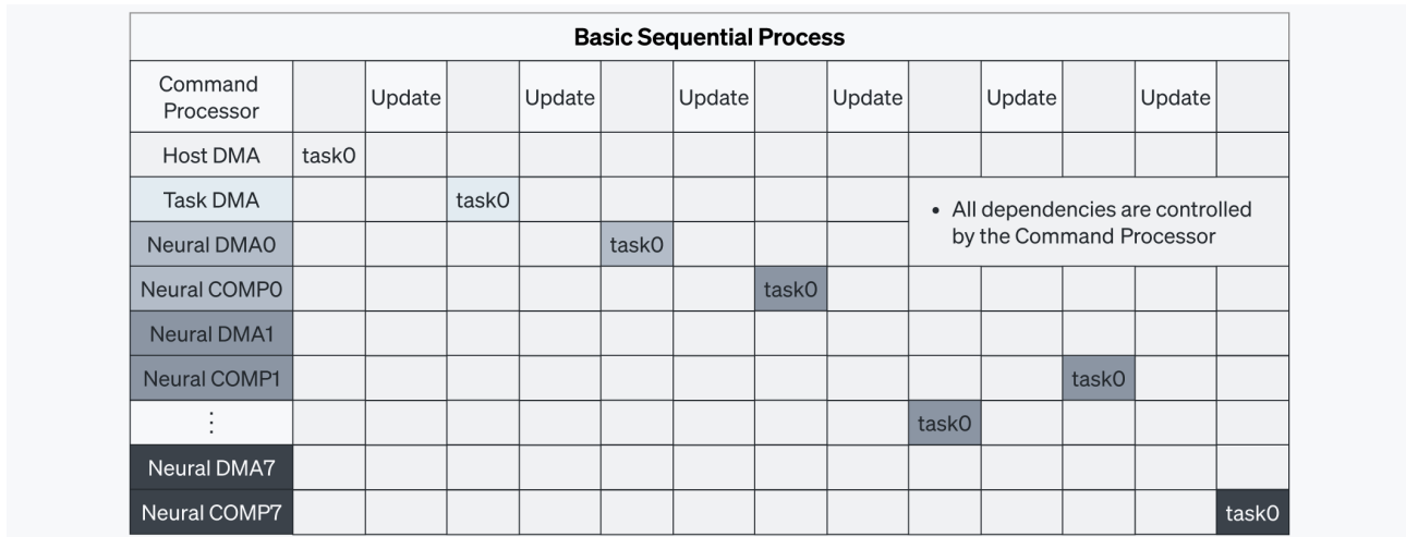
[Figure 5-1. Sequential Execution without Task Managers]
