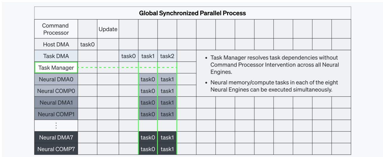
[Figure 5-2. Parallel Execution with Task Managers]
