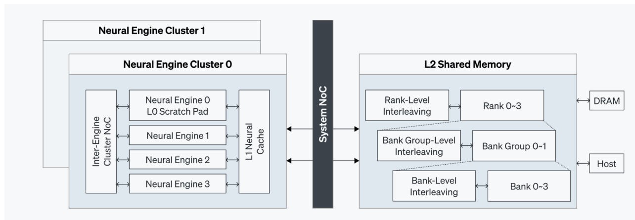
[Figure 3. ATOM™ Hierarchical Memory Subsystem]
