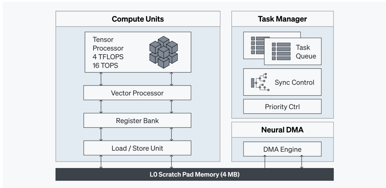
[Figure 2. ATOM™ Neural Engine]
